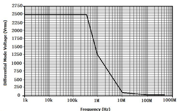
Figure 3:DP6350A Differential Mode Voltage VS Frequency
