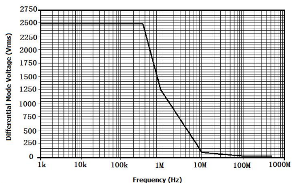
Figure 3:DP6350B Differential Mode Voltage VS Frequency
