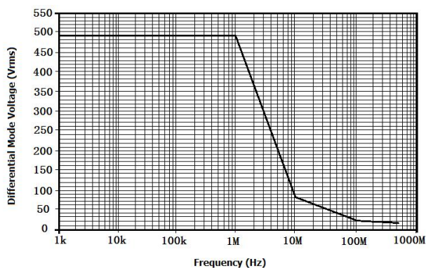
Figure 1:DP6070B Differential Mode Voltage VS Frequency
