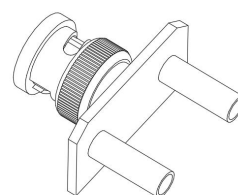
Figure 2 BNC-male-to-banana female-dual
